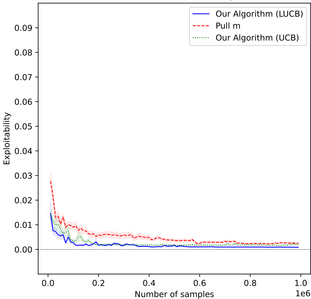
Leduc Poker, Variations, Player o
